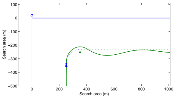
Fig. 10. Helicopter and UAV paths are plotted as solid lines beginning from the bottom. The UAV's desired path is a broken line, and its commanded waypoints are shown. The circle shows the controller's initial estimate of where the helicopter will turn.
