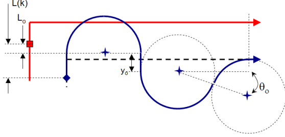
Fig. 4. The fixed curve ( T_2 ) causes constant reduction in lag and transitions smoothly to the convergent rule.
