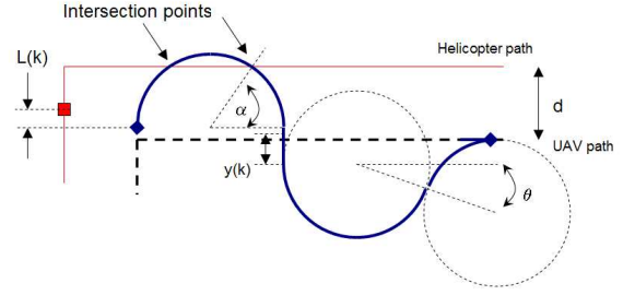
Fig. 7. Two danger points for path rule 3, located at angles \alpha and \pi - \alpha .
